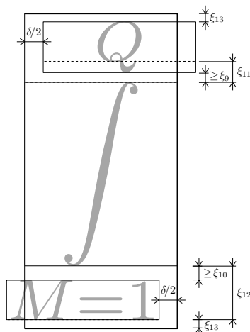
Figure 1: \text{\TeX} font metric parameters affecting the placement of limits above or below big operators.
