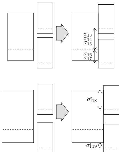
Figure 4: \text{\TeX} font metric parameters affecting the placement of superscripts and subscripts on a simple character or a boxed subformula.
