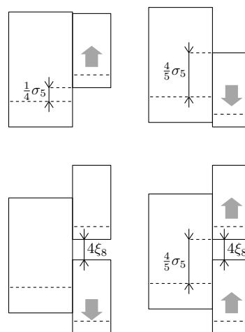
Figure 5: \text{\TeX} font metric parameters affecting the placement of superscripts and subscripts in cases of resolving collisions.
