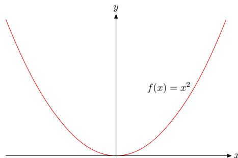
Figure 9: Labeling text
