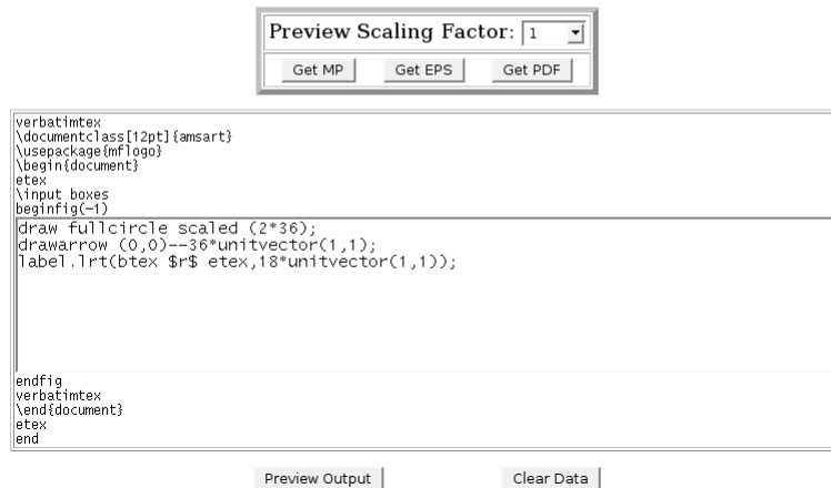
Figure 2: METAPOST Previewer
