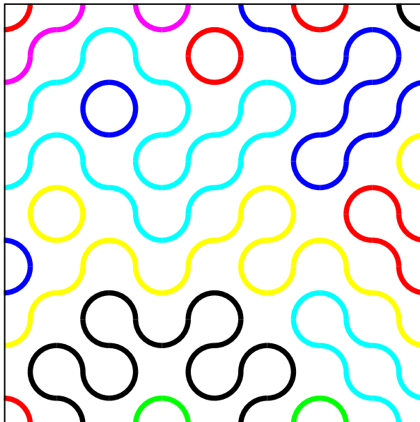
Figure 4: Problem 2: TRUCHET's tiling (8x8)
