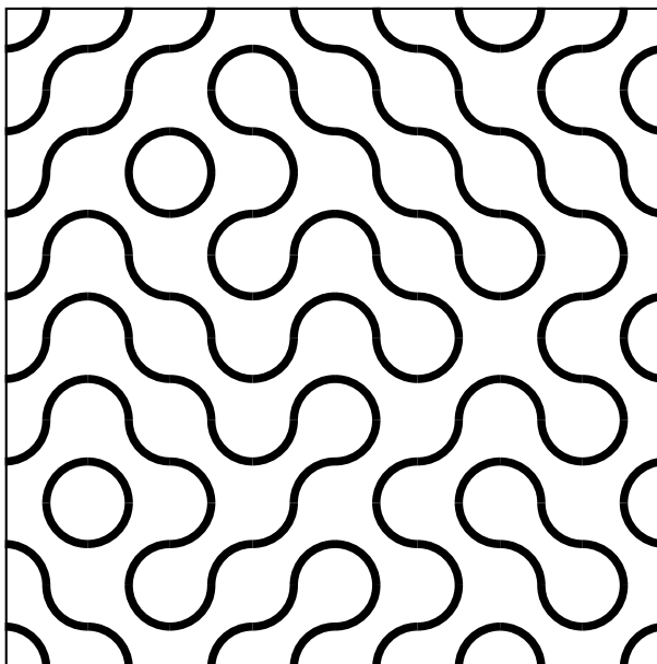
Figure 2: Problem 1: TRUCHET's tiling (8x8)
