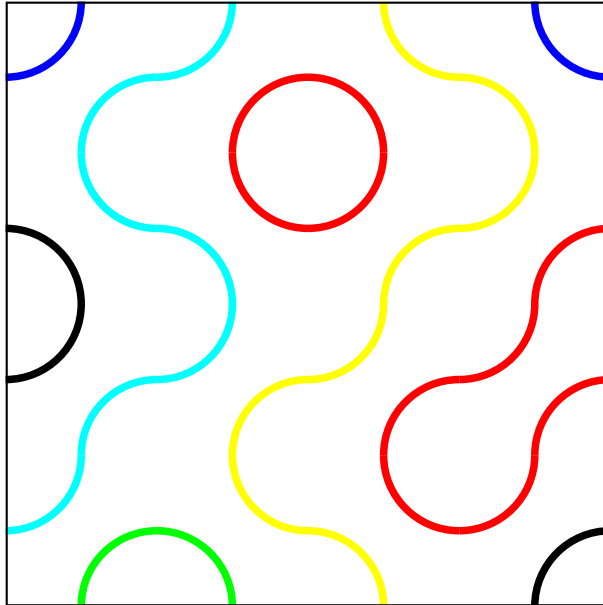
Figure 3: Problem 2: TRUCHET's tiling (4x4)
