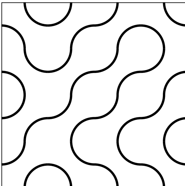
Figure 1: Problem 1: TRUCHET's tiling (4x4)
