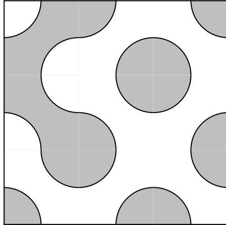
Figure 5: Problem 3: TRUCHET's tiling (3x3)
