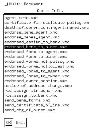
Figure 6: Top-level window of the T E Xmerge application.
