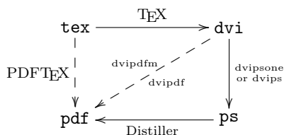
Figure 1: From \TeX to PDF
